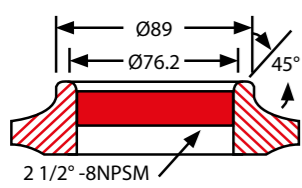
Detail 2 1/2° Thread
