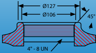
Detail 4" Thread
